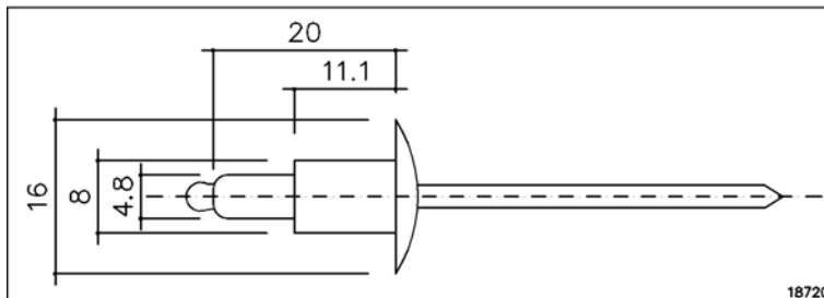
ASTRO rivet with fixed cylinder for ETER-COLOR
